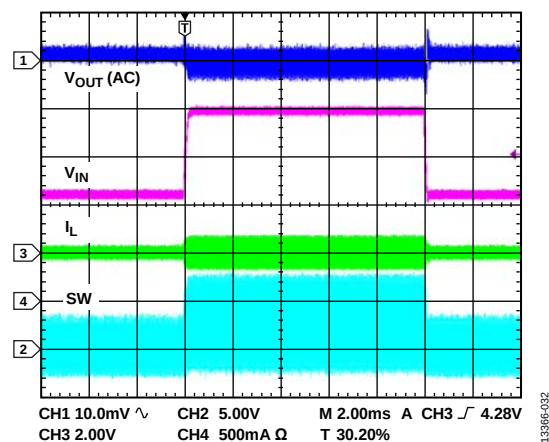
Figure 32. Line Transient of PWM Mode, I_{LOAD} = 500 \text{ mA} ( I_L is the Inductor Current)
