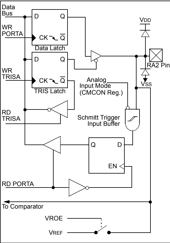
FIGURE 5-2: BLOCK DIAGRAM OF RA2/AN2/VREF PIN
