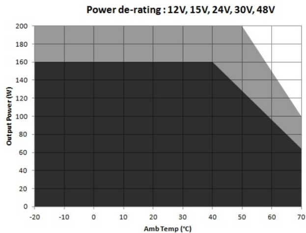
Figure 1. Derating Curves
