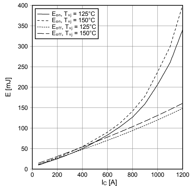
Schaltverluste IGBT-Wechselr. (typisch) switching losses IGBT-inverter (typical) E_{on} = f(I_c), E_{off} = f(I_c) V_{GE} = \pm 15\text{ V}, R_{Gon} = 1.5\ \Omega, R_{Goff} = 1.5\ \Omega, V_{CE} = 600\text{ V}
