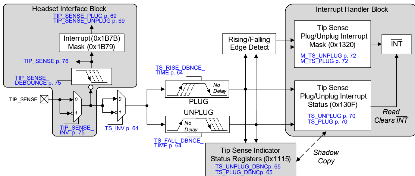
Figure 4-24. Tip-Sense Controls
