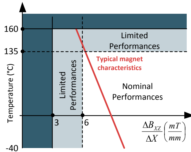
fig. 9 - Minimum useful signal definition for linear stray-field immune application
