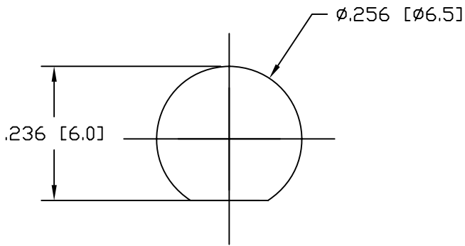
RECOMMENDED MOUNTING HOLE DIMENSIONS
