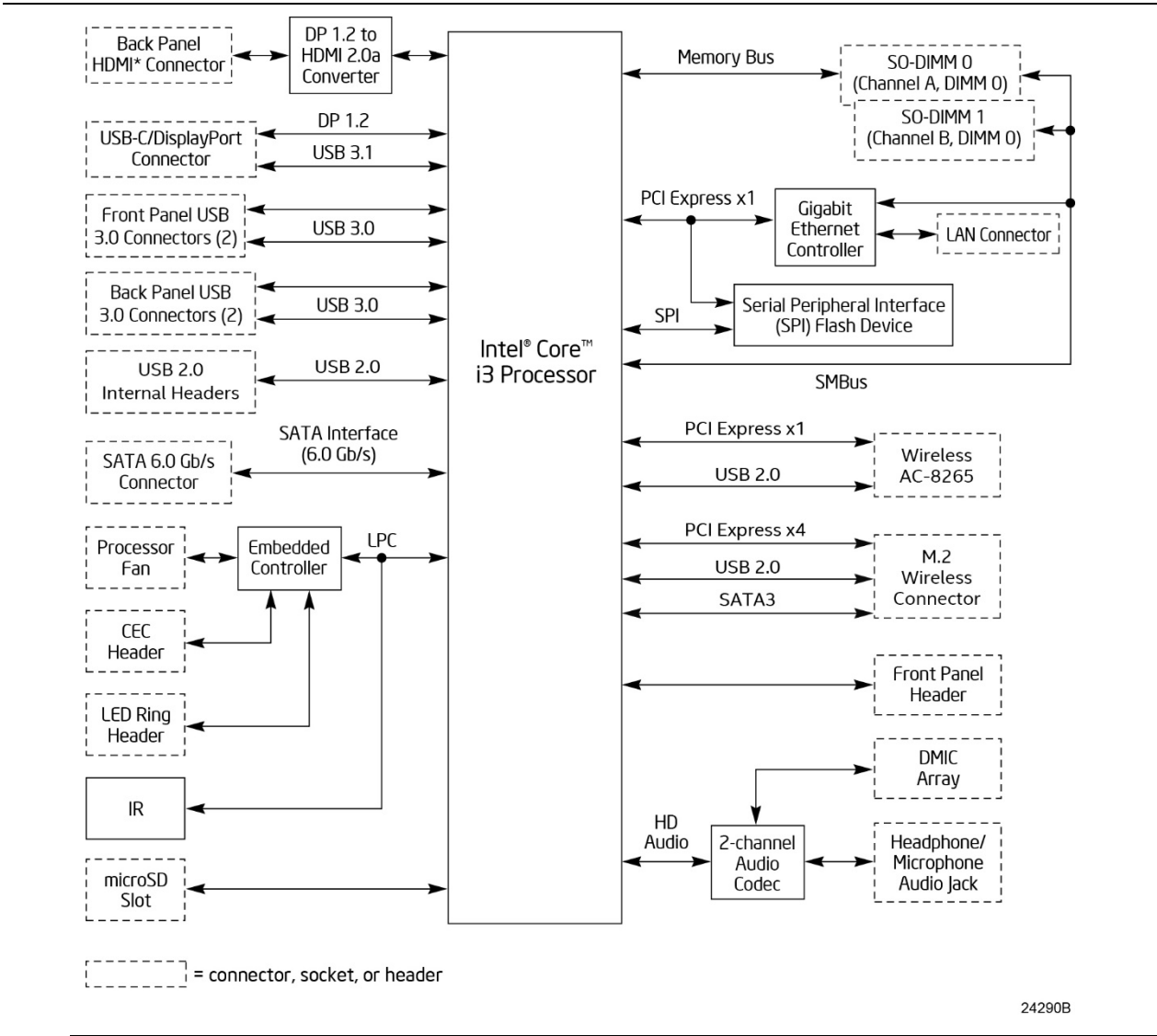
Figure 3. Block Diagram
