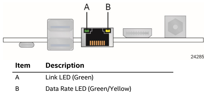
Figure 6. LAN Connector LED Locations
