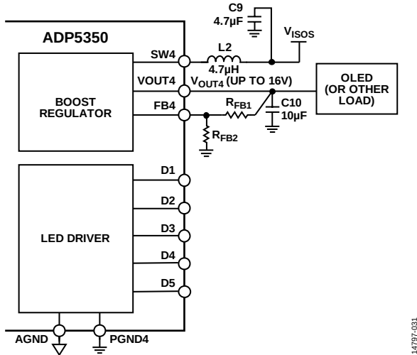
Figure 48. Boost Regulator in Standalone Operation Mode
