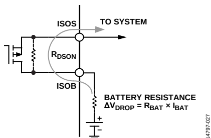
Figure 44. Discharge Current Sensing Through Battery Isolation FET
