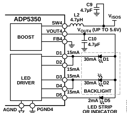
Figure 53. Two LEDs in Parallel (30 mA each) for Grouped Backlight and One LED Strip or Indicator (2 mA)
