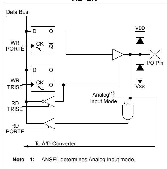
FIGURE 3-21: BLOCK DIAGRAM OF RE<2:0>
