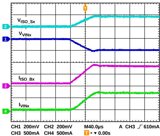
Figure 22. Input Current-Limit Transition from 100 mA to 900 mA, ISO\_Sx Load = 66 \Omega , Charging = 750 mA
