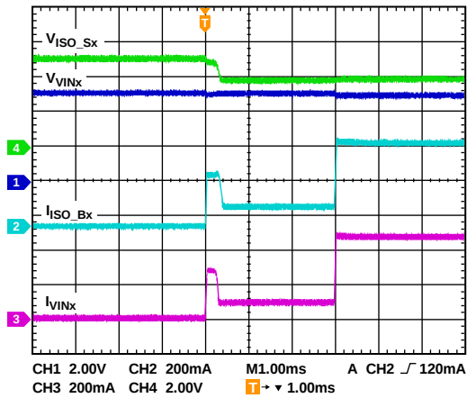
Figure 20. Charging Startup, V_{VINx} = 5.0\text{ V} , ILIM[3:0] = 0110 (Binary) = 500 mA, ICHG[4:0] = 01110 (Binary) = 750 mA
