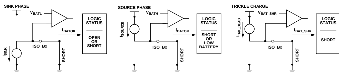
Figure 28. Trickle Charge
