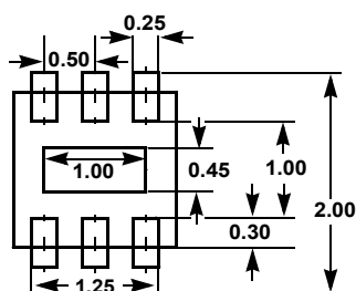
LAND PATTERN 6
