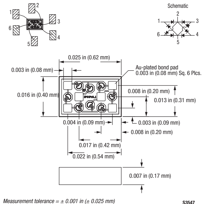
Figure 6. 588-065 Package Dimensions
