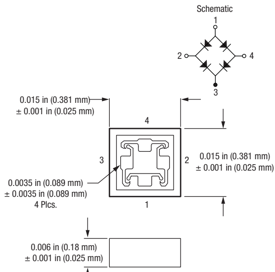
Figure 7. 551-004 Package Dimensions
