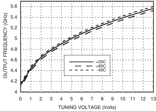
RFOUT/2 Frequency vs. Tuning Voltage, Vcc = +5V
