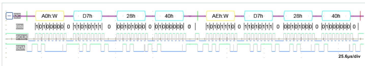
Figure 7 — DISABLE_FAULT COMMAND (D7h)_WRITE
