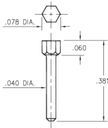
8979-0-00-XX-00-00-03-0 Hex press-fit in .074 plated thru hole
