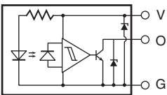
Internal circuit
