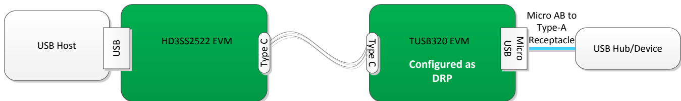
Figure 3. Example Configuration Using HD3SS2522 and TUSB320 EVMs
