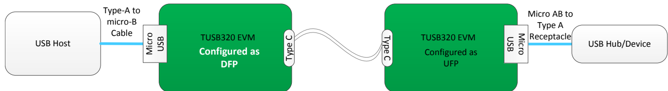
Figure 2. Example Configuration Using Two TUSB320 EVMs
