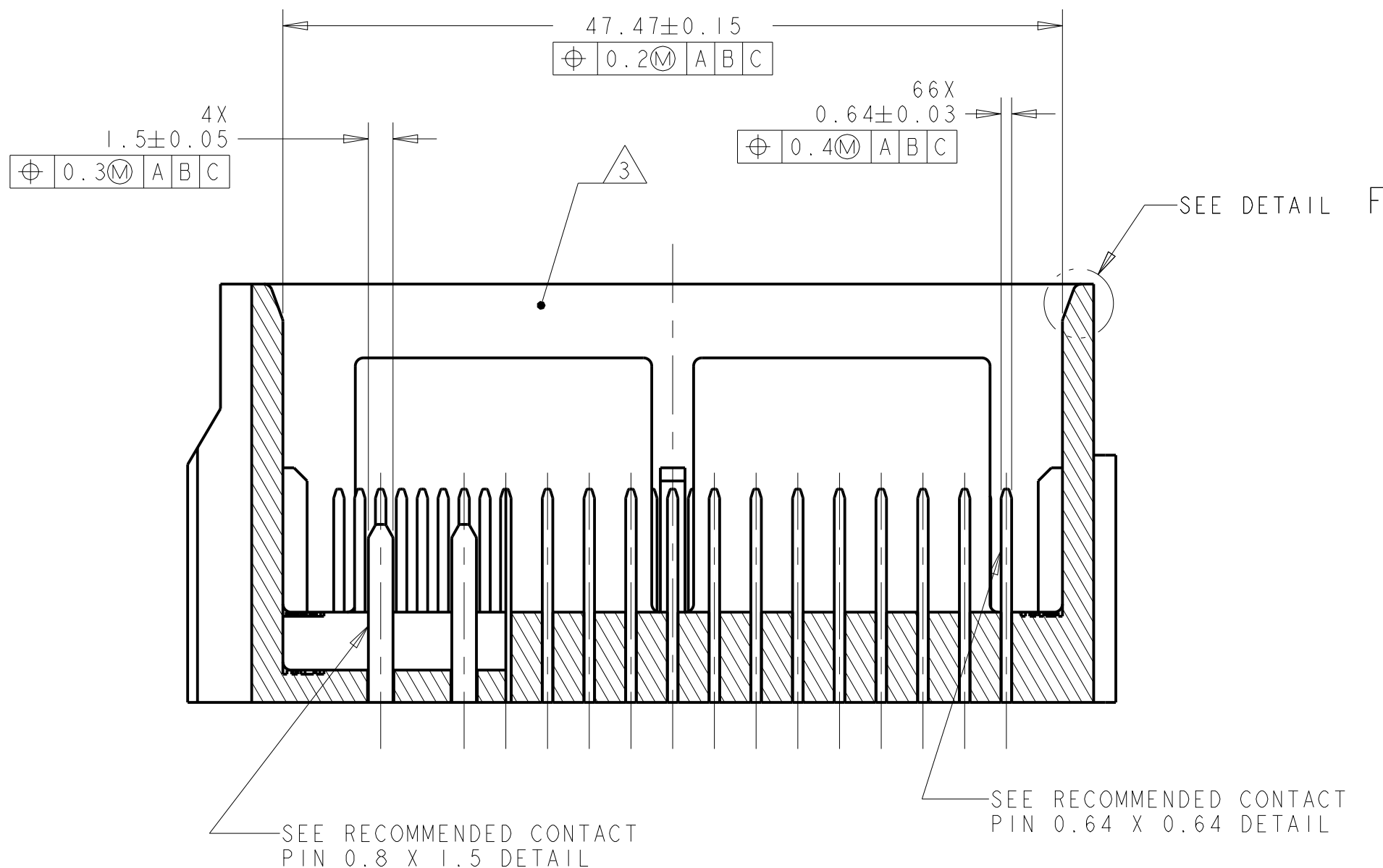
SECTION B-B
