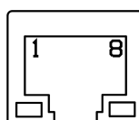
Figure 6: RS422 connector
