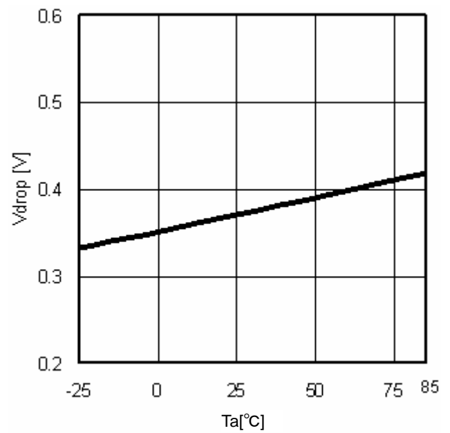
Fig.17 Minimum dropout Voltage1 ( V_{CC}=5\text{V} , I_O=-0.5\text{A} )
