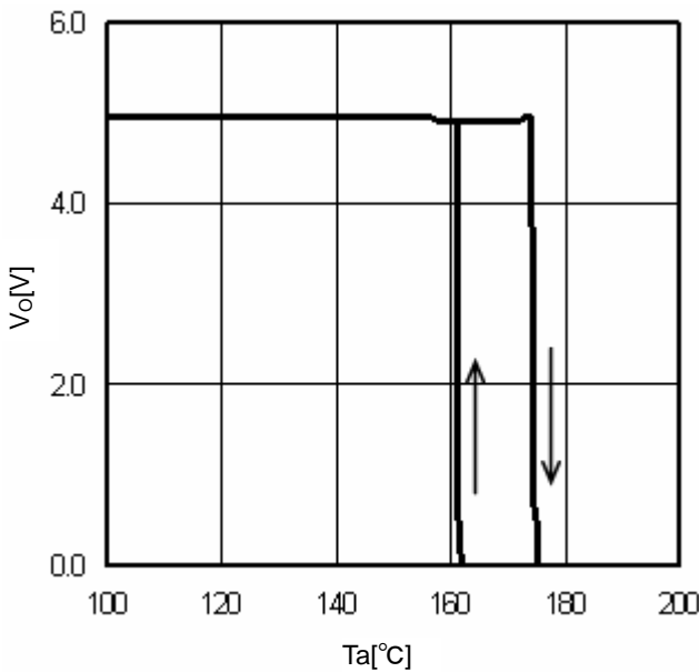
Fig.15 TSD ( I_o=0mA )
