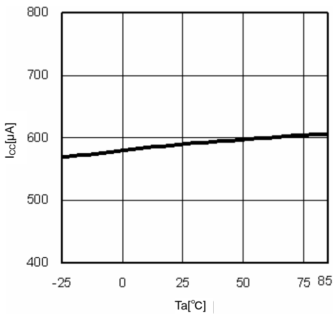
Fig.9 T_a - I_{cc}
