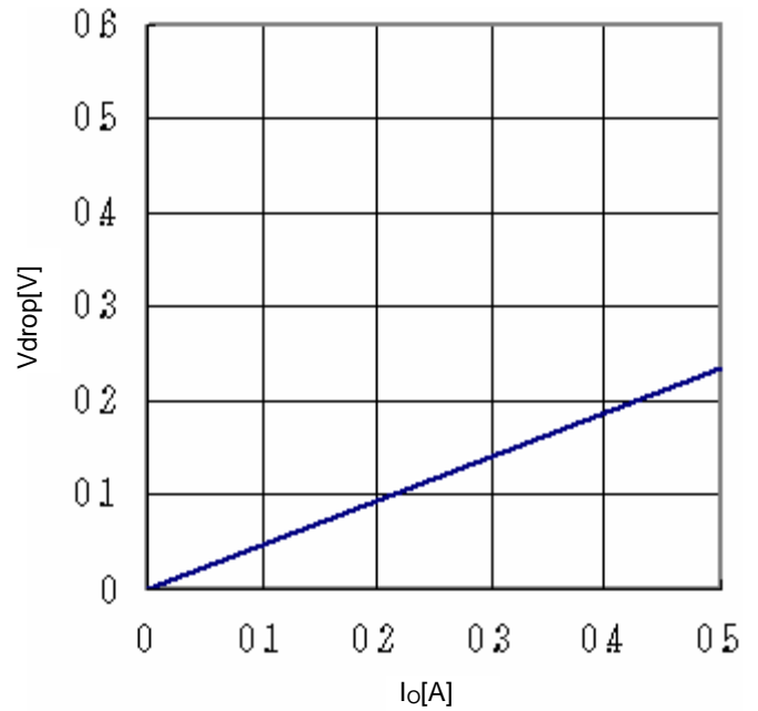
Fig.25 Minimum dropout Voltage 6 (V CC =12V、Ta=25°C)
