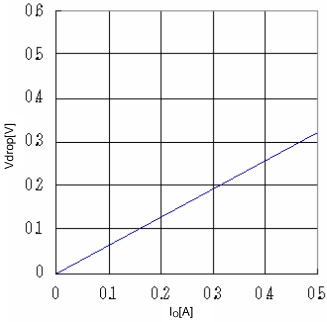
Fig.22 Minimum dropout Voltage 3 (V CC =6V、Ta=25°C)
