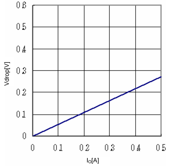
Fig.23 Minimum dropout Voltage 4 (V CC =8V、Ta=25°C)
