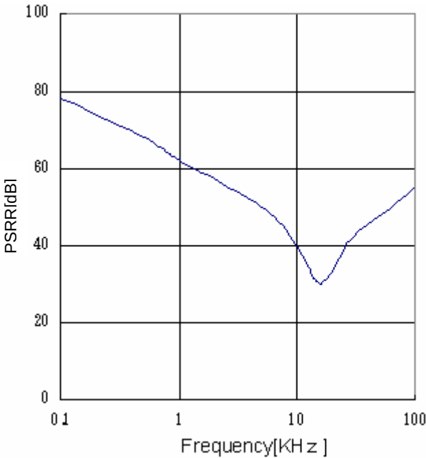
Fig.20 PSRR ( I_o=0mA )
