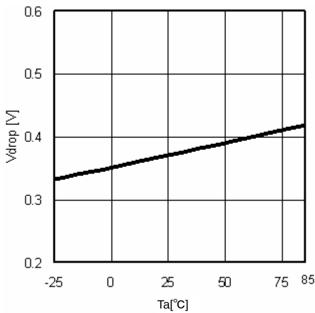
Fig.17 Minimum dropout Voltage1 ( V_{cc}=5V , I_o=-0.5A )
