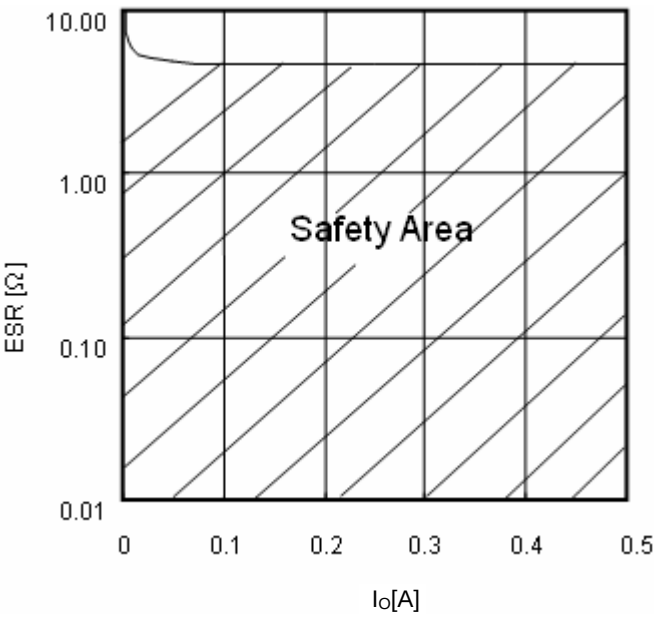
Fig.18 ESR condencer
