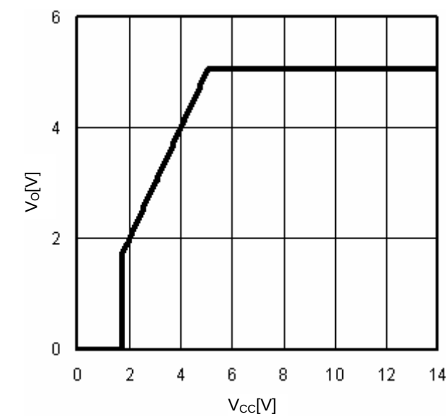
Fig.14 V_{cc}-V_o ( I_o=0mA )
