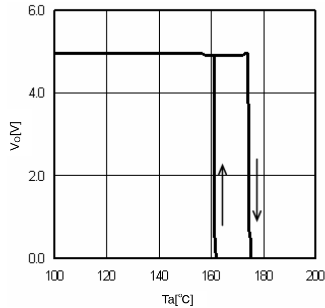
Fig.15 TSD ( I_o=0mA )
