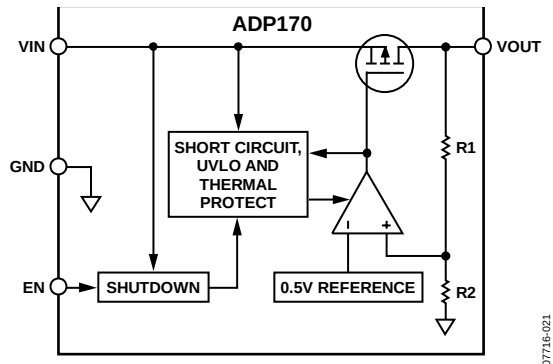
Figure 25. ADP170 Internal Block Diagram
