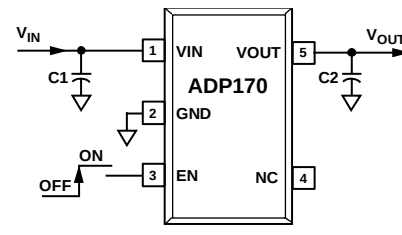
Figure 1. ADP170 with Fixed Output Voltage, 1.8 V
