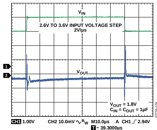
Figure 24. Line Transient Response, Load Current = 300 mA
