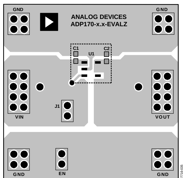
Figure 40. Example ADP170 PCB Layout
