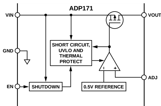
Figure 26. ADP171 Internal Block Diagram
