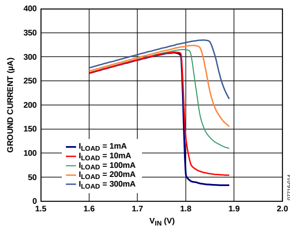
Figure 14. Ground Current vs. Input Voltage (In Dropout)
