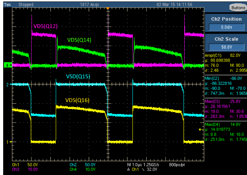
Figure 4. Stresses ( V_{PORT} = 57V , 5V/13A)
