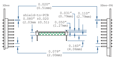
(Side Views)
