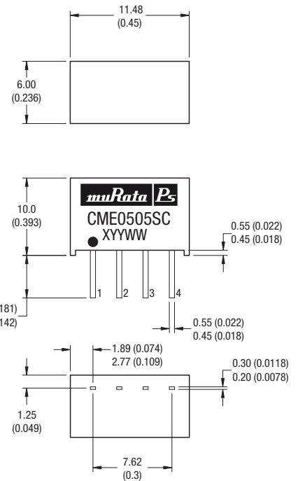
SC Package
