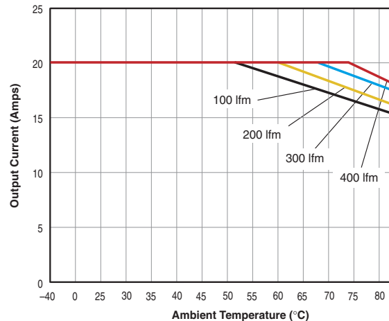
ULE-3.3/20-D48 Maximum Current Temperature Derating (VIN = 48V, air flow direction is transverse)
