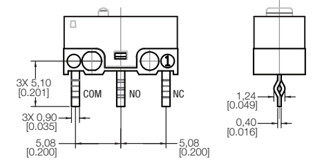
TYPE 30 - PCB SNAP-IN
