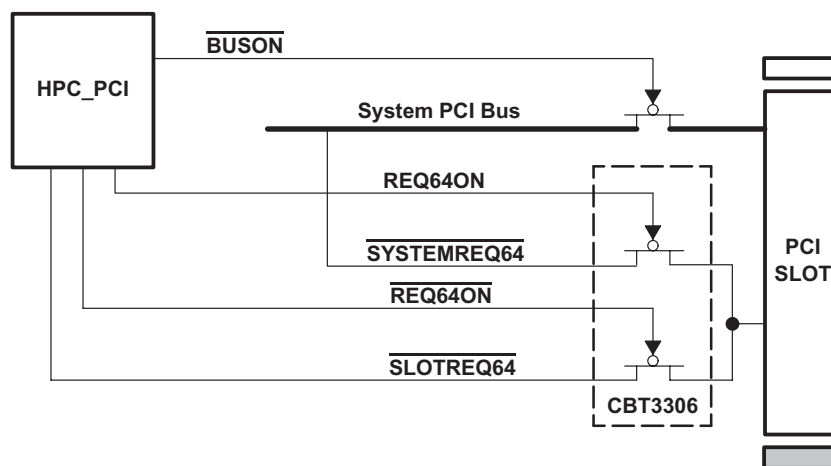
Figure 12. \text{SLOTREQ64} Implementation Using CBT3306
