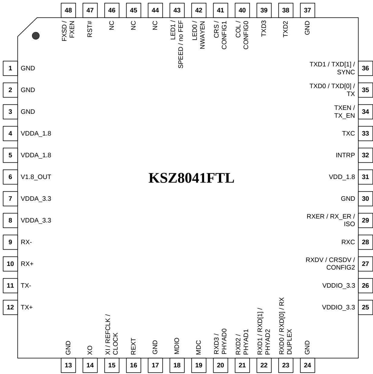
48-Pin TQFP
