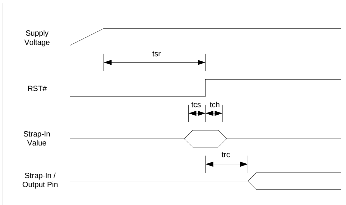
Figure 20. Reset Timing
