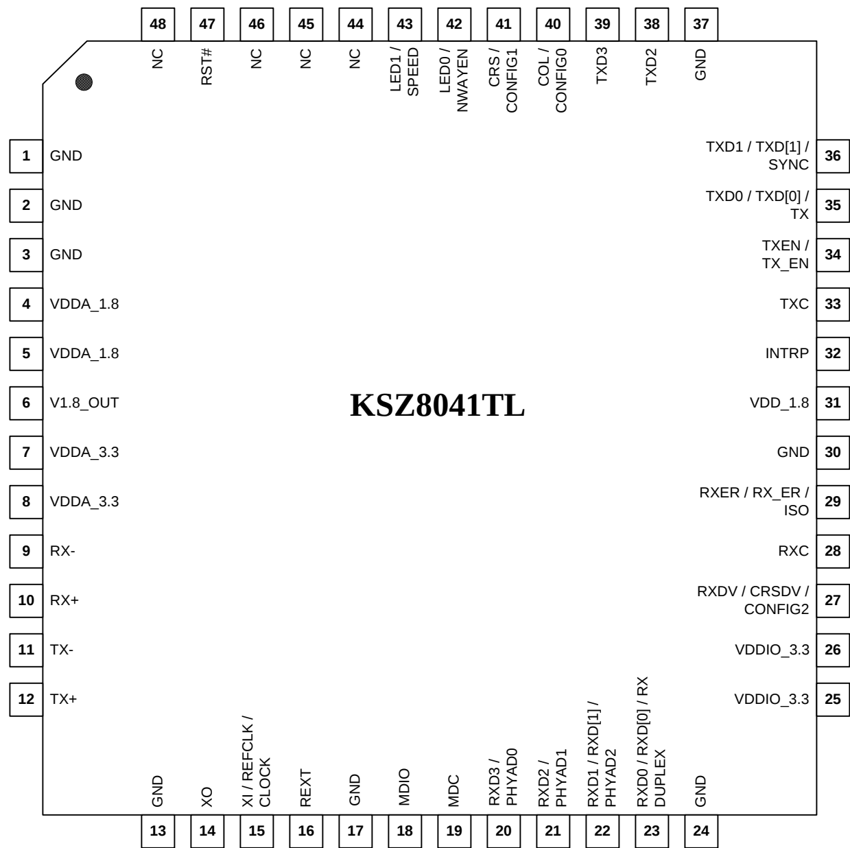
48-Pin TQFP
