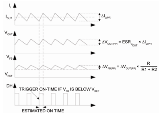
Figure 2. MIC2176 Control Loop Timing
