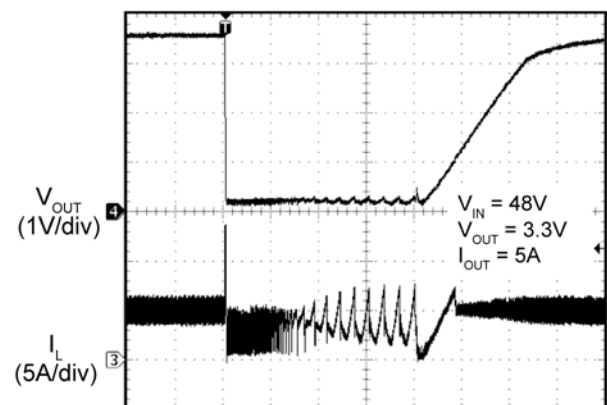
Time (2ms/div)
