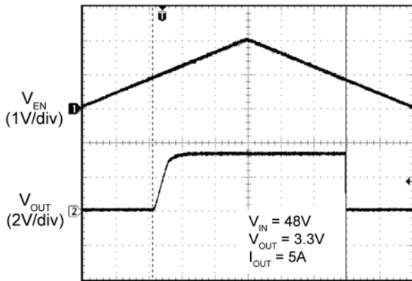
Time (10ms/div)
