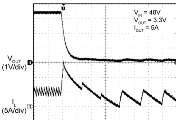
Time (20μs/div)
