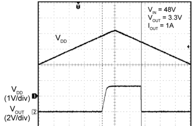
Time (20ms/div)
