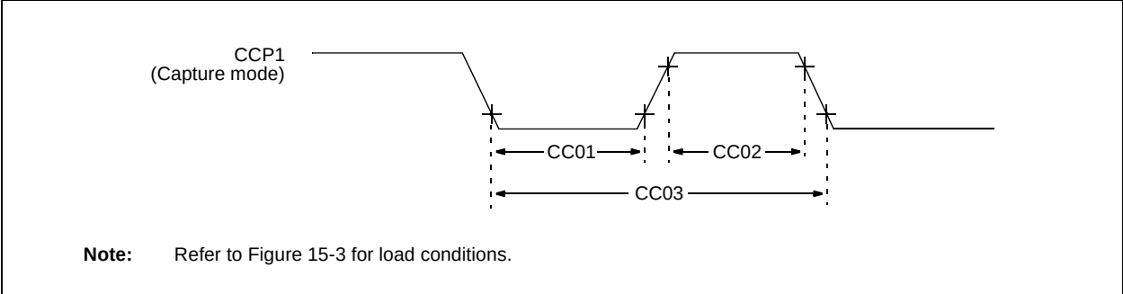
FIGURE 15-9: CAPTURE/COMPARE/PWM TIMINGS (ECCP)
