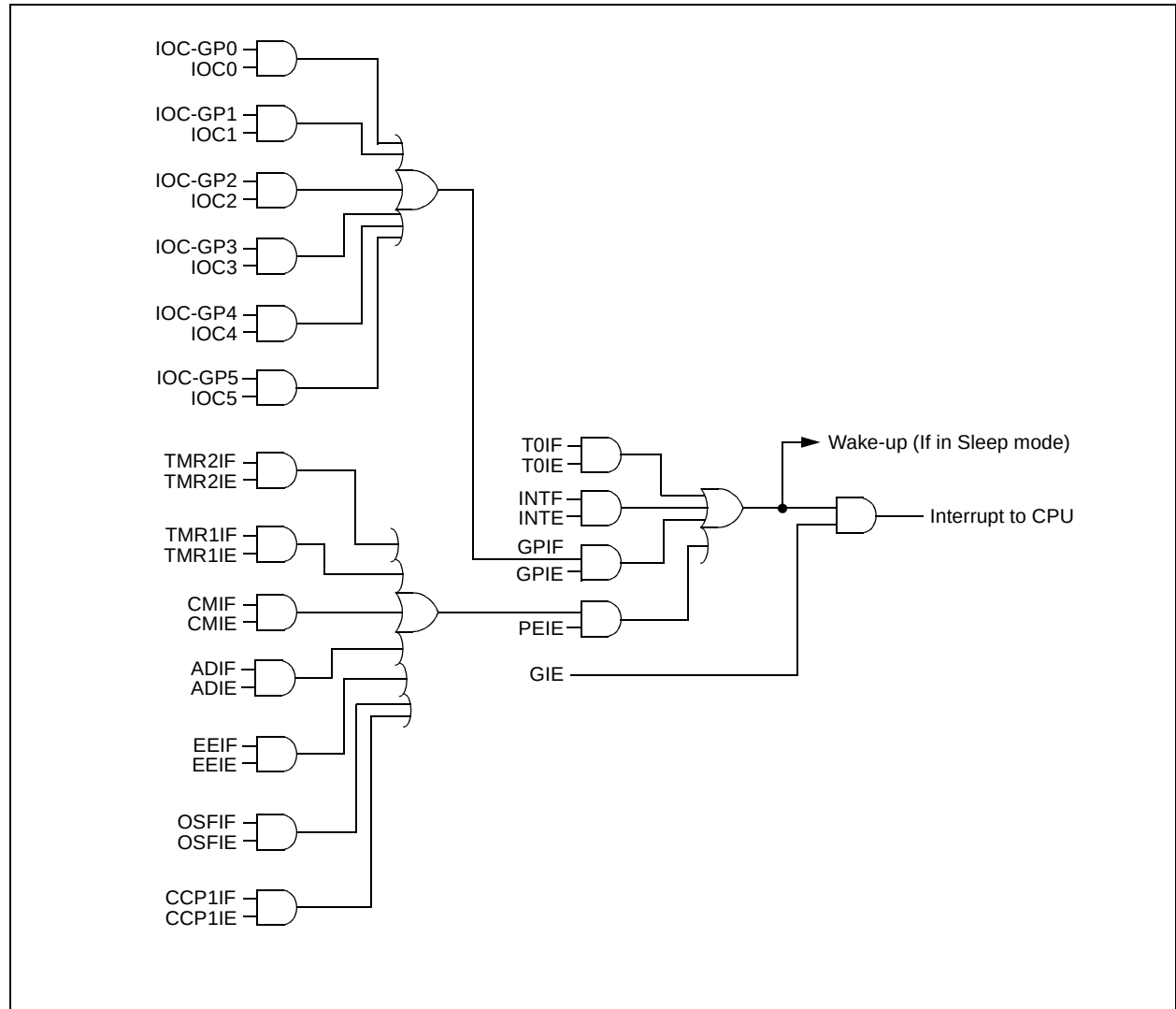
FIGURE 12-7: INTERRUPT LOGIC
