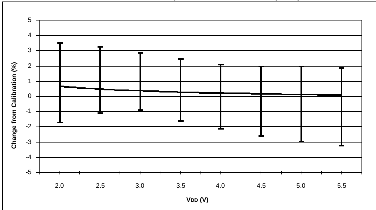
FIGURE 16-40: TYPICAL HFINTOSC FREQUENCY CHANGE vs. V_{DD} ( -40^{\circ}\text{C} )
