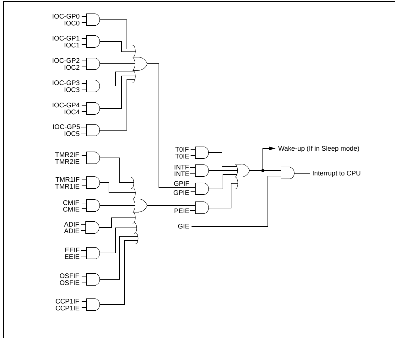
FIGURE 12-7: INTERRUPT LOGIC
