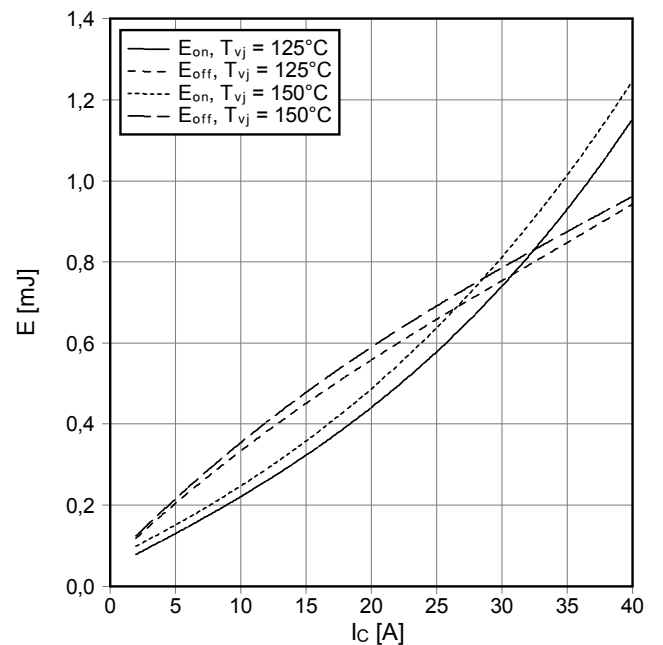
Schaltverluste IGBT-Wechselr. (typisch) switching losses IGBT-inverter (typical) E_{on} = f(I_C), E_{off} = f(I_C) V_{GE} = \pm 15 \text{ V}, R_{Gon} = 18 \Omega, R_{Goff} = 18 \Omega, V_{CE} = 300 \text{ V}
