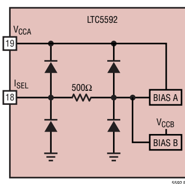
Figure 12. I_{SEL} Interface Schematic
