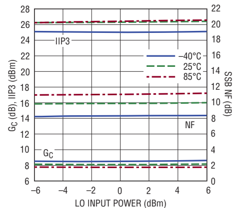
2550MHz Conversion Gain, IIP3 and NF vs LO Power
