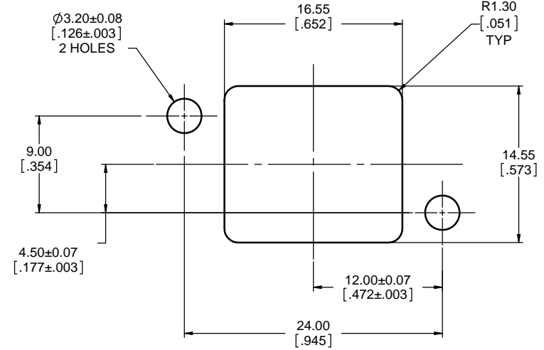
RECOMMENDED PANEL CUTOUT OUTSIDE PANEL VIEW
