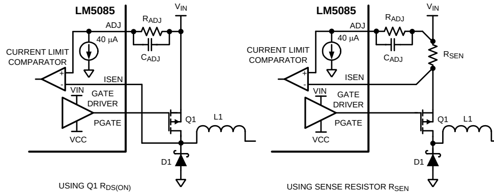
Figure 26. Current Limit Sensing
