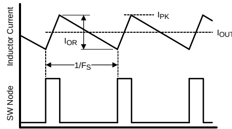
Figure 27. Inductor Current Waveform
