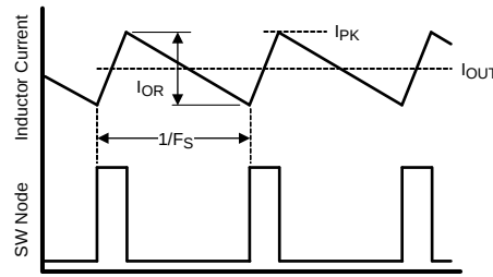
Figure 27. Inductor Current Waveform
