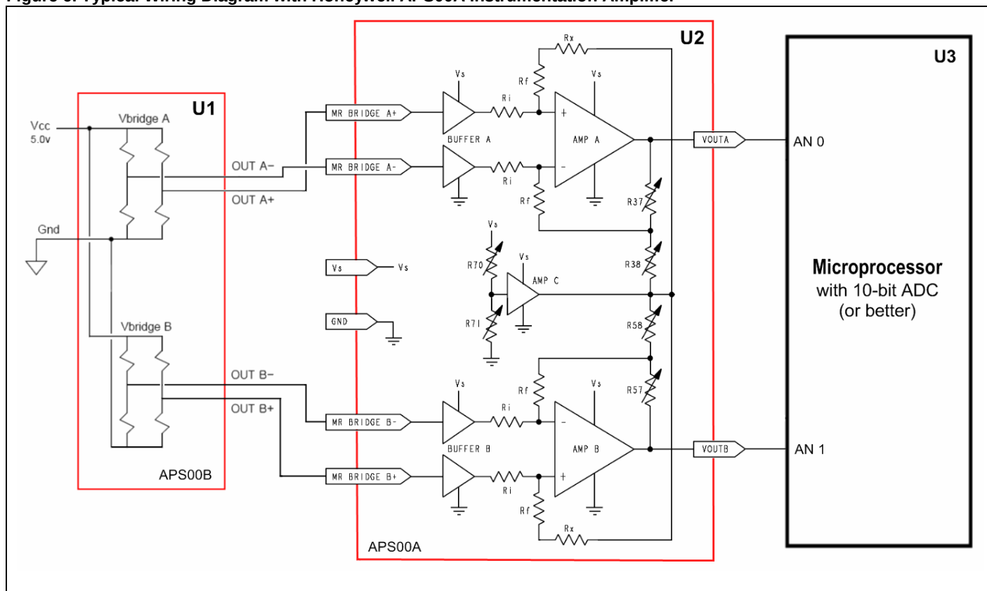
Figure 6. Typical Wiring Diagram with Honeywell APS00A Instrumentation Amplifier
