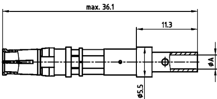
Socket contact/Screw crimp
