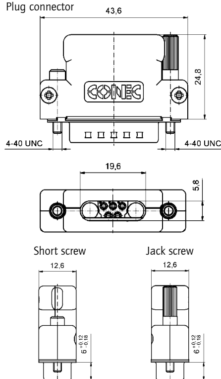
Plug connector
