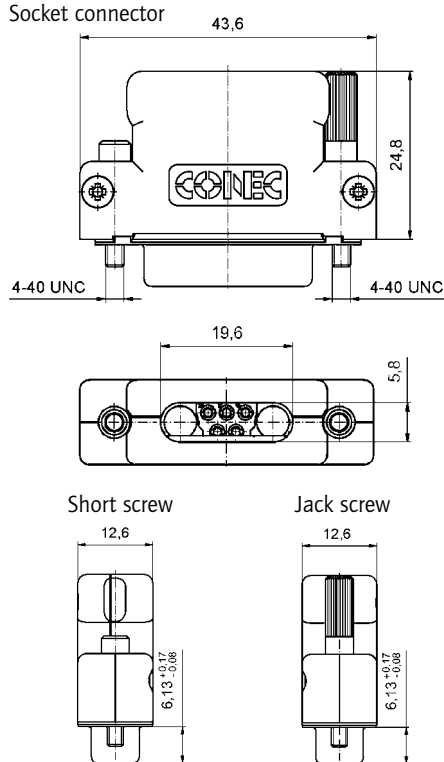
Socket connector
