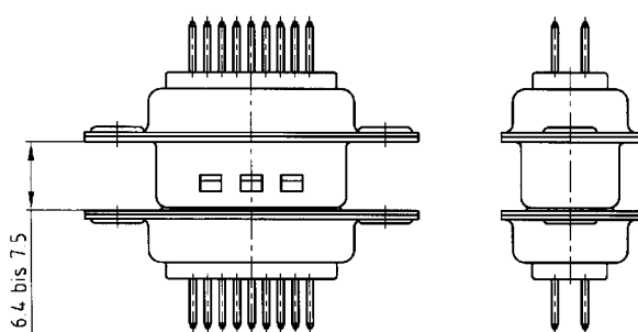
Rigid mount vertical to tolerance guide
