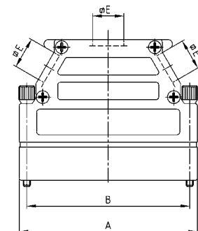
Cable clamp
