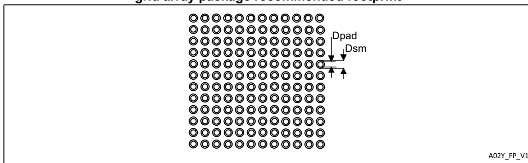
Figure 78. UFBGA144 - 144-pin, 10 x 10 mm, 0.80 mm pitch, ultra fine pitch ball grid array package recommended footprint
