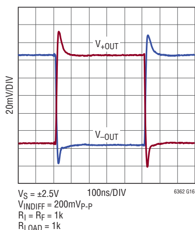
Small-Signal Step Response
