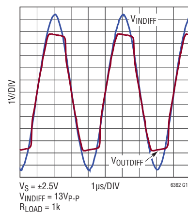
Overdriven Output Transient Response
