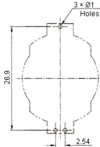
PCB Mounting Layout
