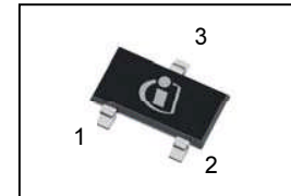
PG-SC59
